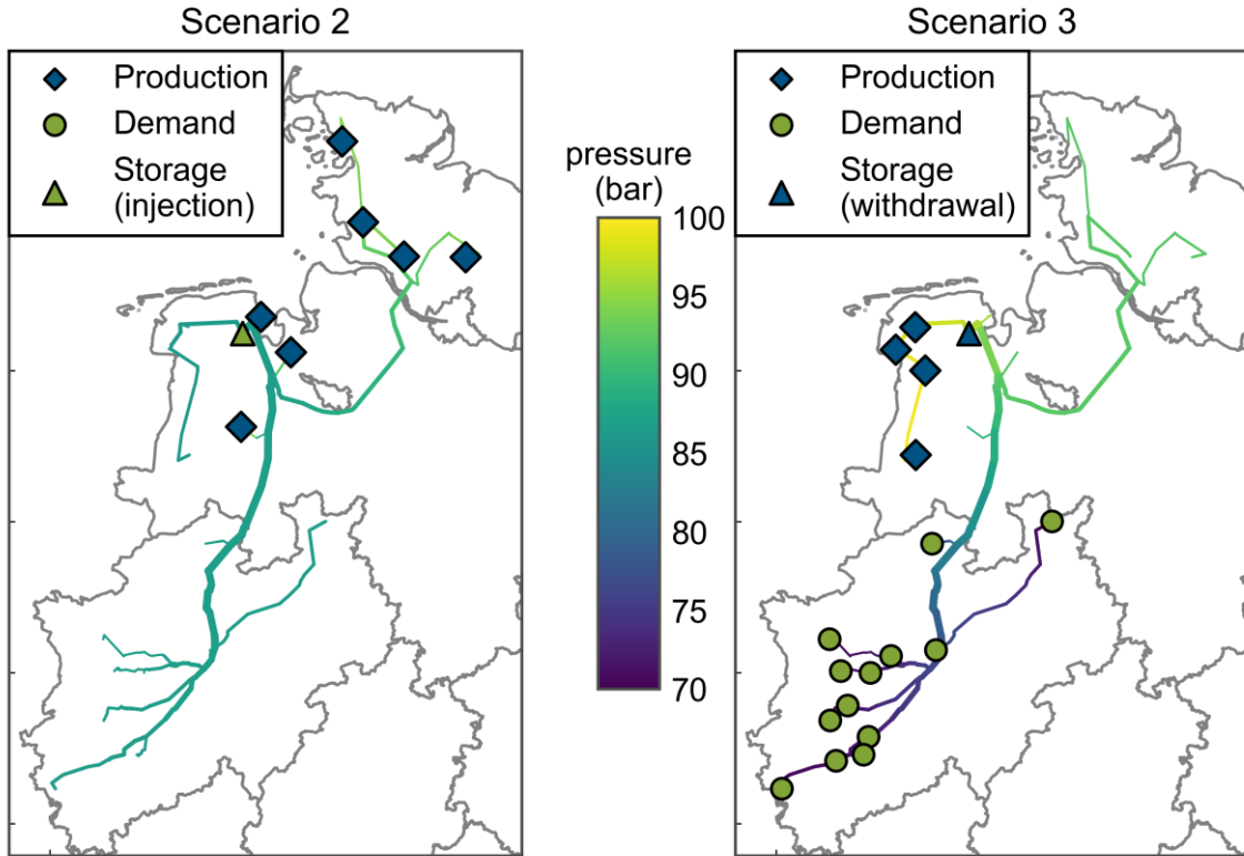
Figure 11. Exemplary pressure gradients of the tree network for scenario 2 (lowest pressure gradient) and scenario 3 (largest pressure gradient).
